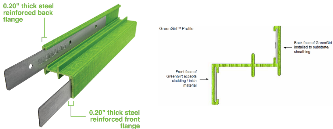
Figure 2. GreenGirt
