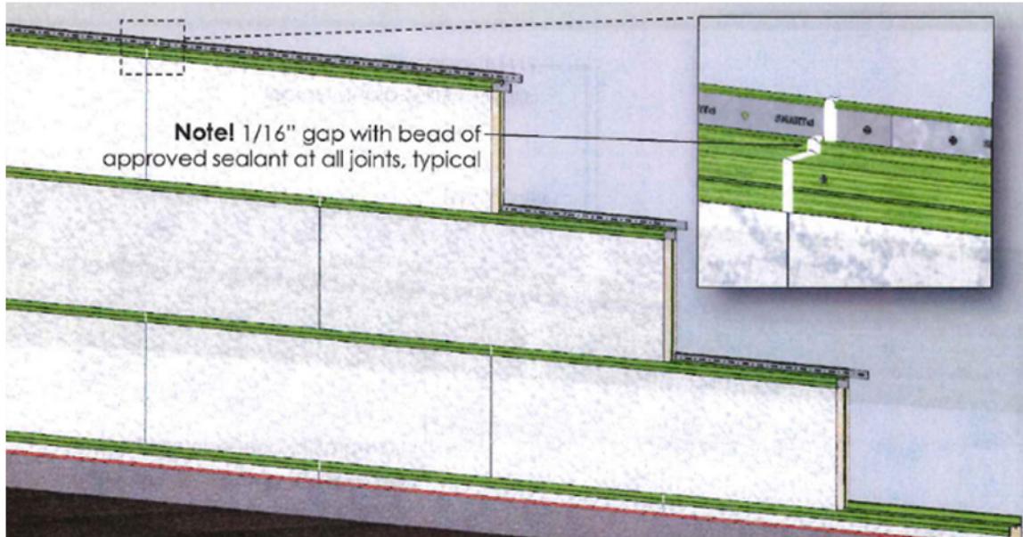
Figure 6. Installation Detail
